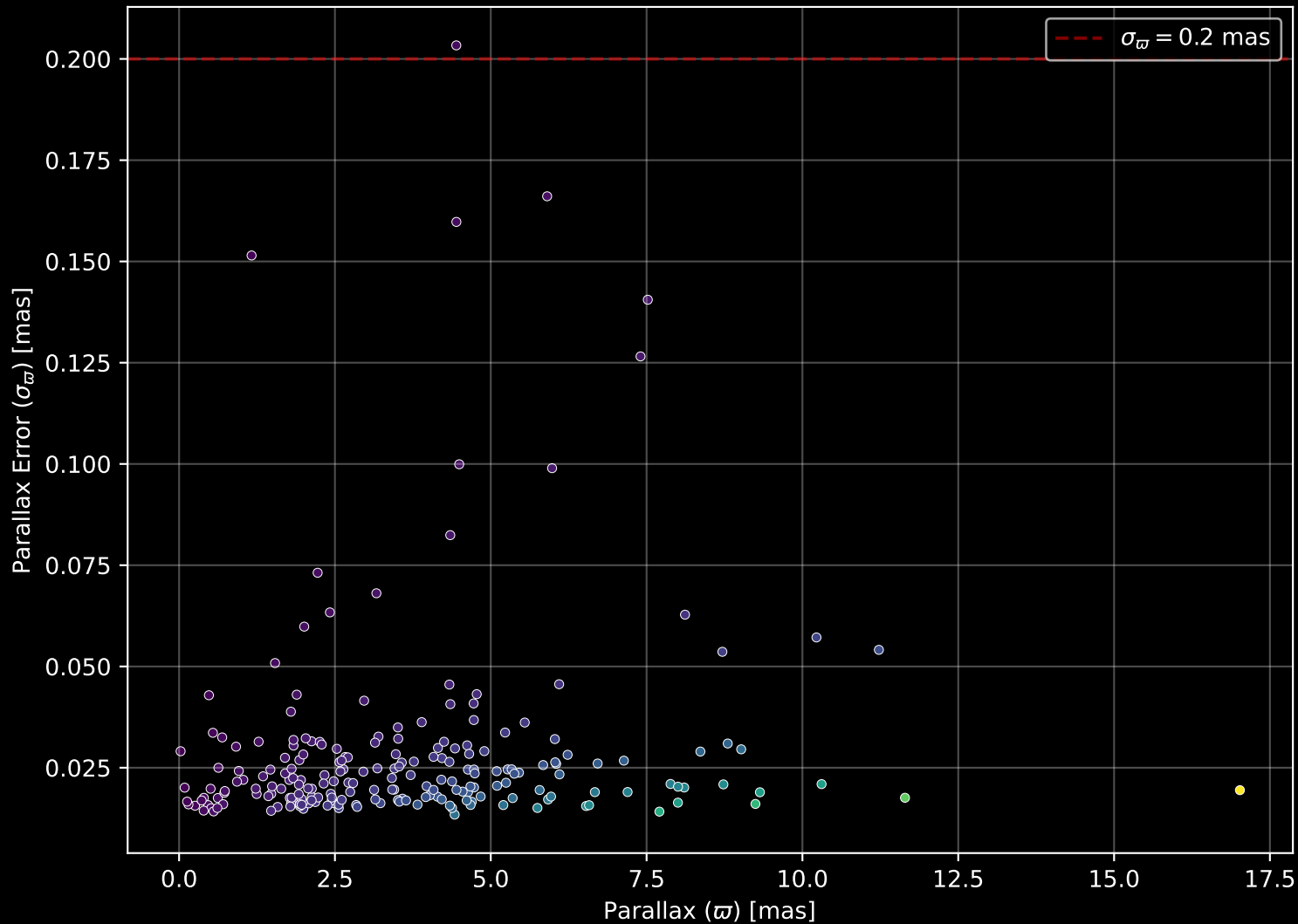
APOGEE DR17 Field: [056+88_MGA] Parallax Quality (n= 217)
