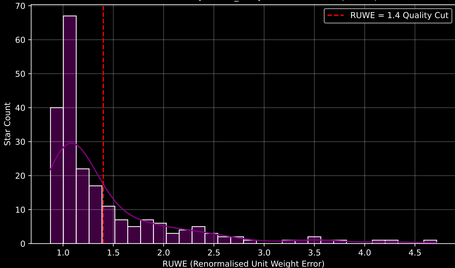
GAPOGEE DR17 Field [056+88_MGA] RUWE Distribution (n= 211)
