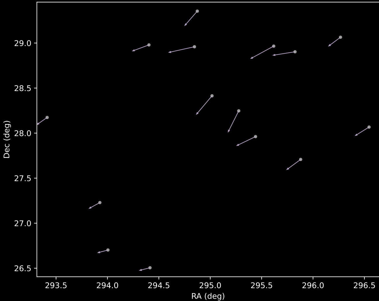
APOGEE DR17 Cluster 9 Proper Motion Vectors (n=15)
