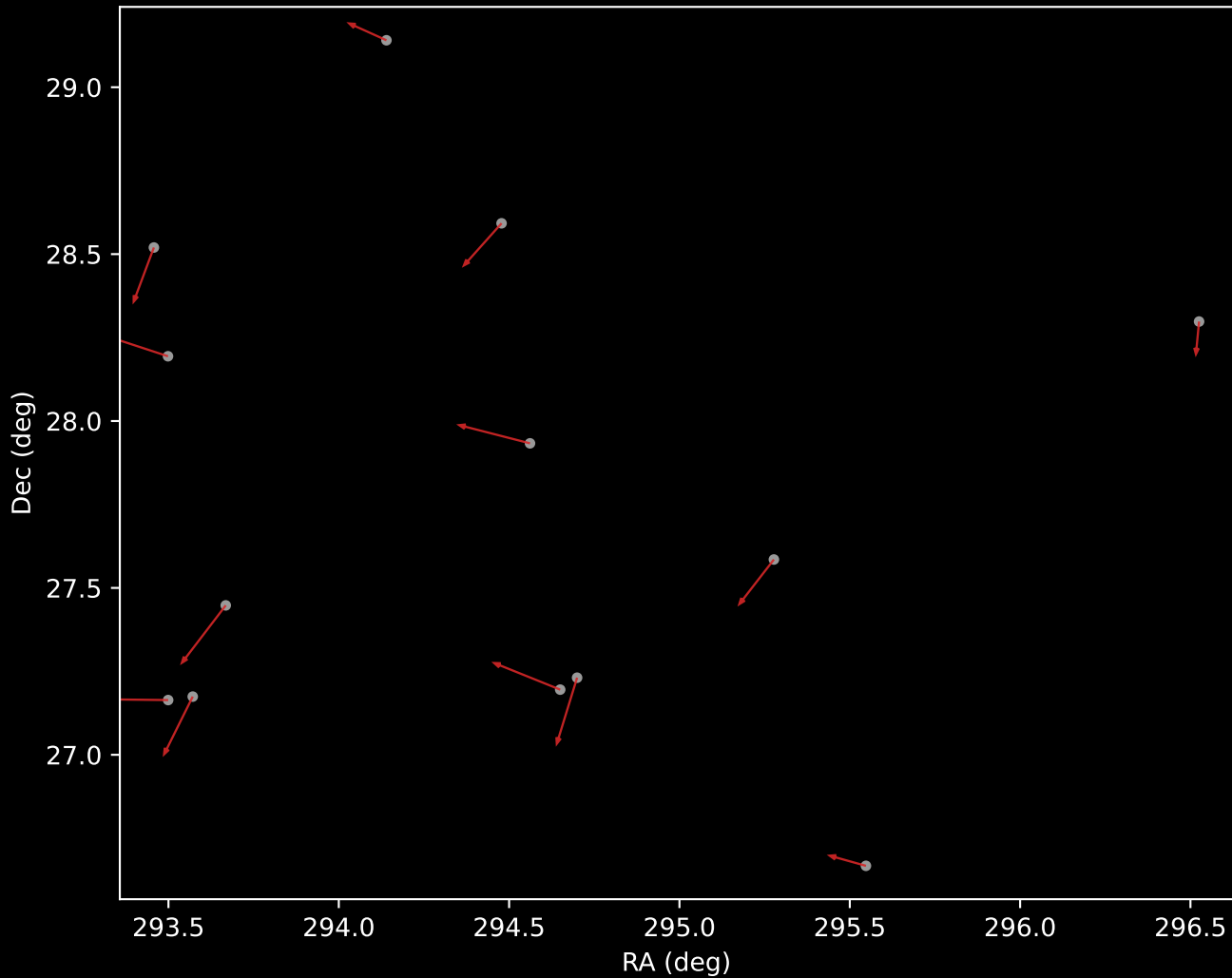
APOGEE DR17 Cluster 6 Proper Motion Vectors (n=13)
