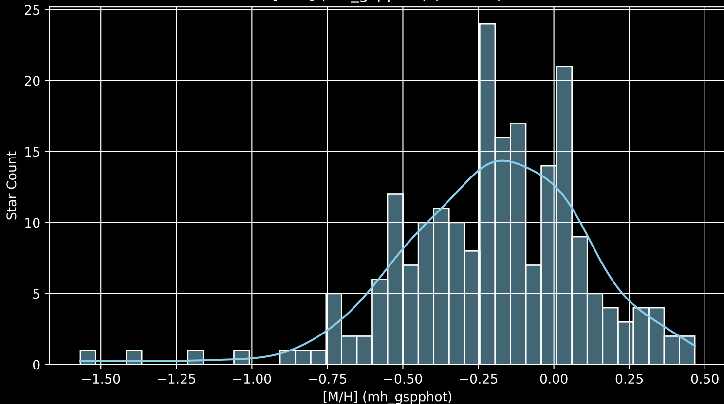
APOGEE DR17 Field: [056+88_MGA [M/H] (mh_gspphot) (n= 212)
