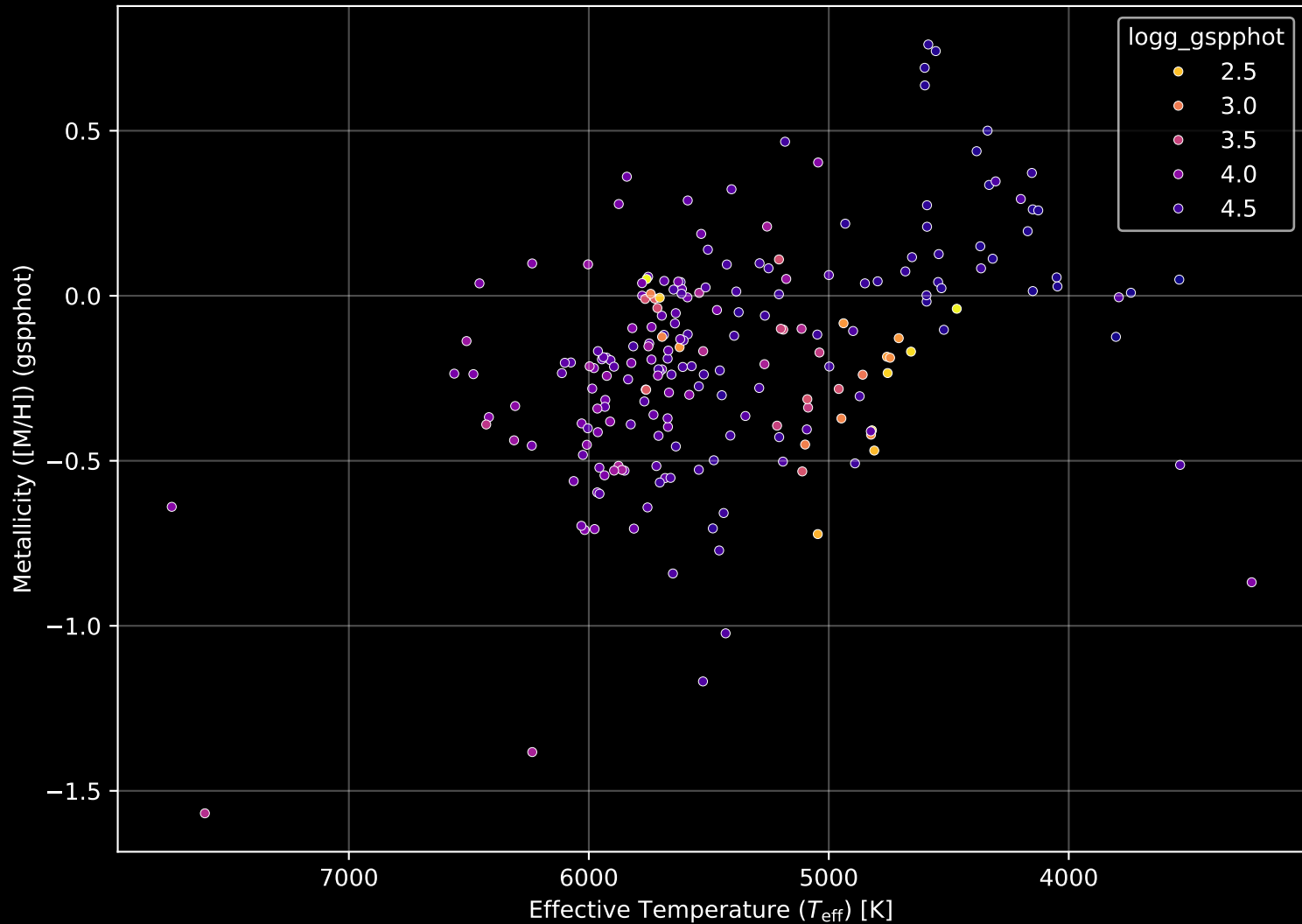
APOGEE DR17 Field: [056+88_MGA] Stellar Population Parameters (n= 217)
