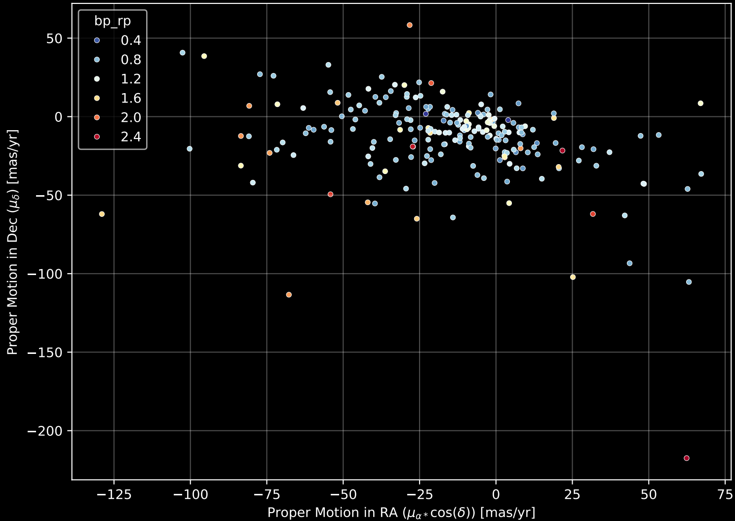
APOGEE DR17 Field: [056+88_MGA] Proper Motion Diagram (n= 217)
